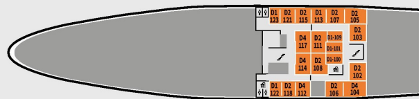
DECK C
